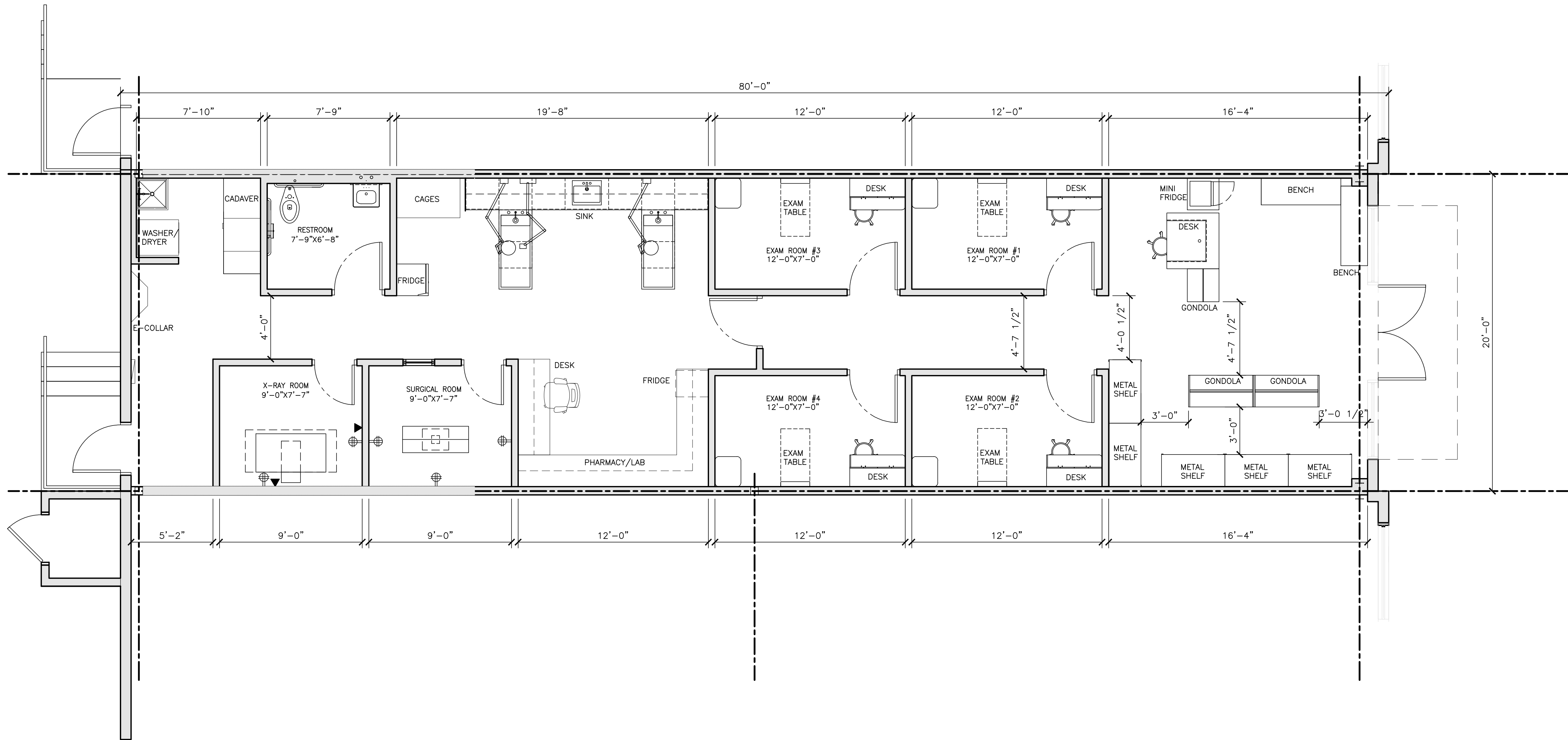
1 FLOOR PLAN A1.0 1/4" = 1'-0"
