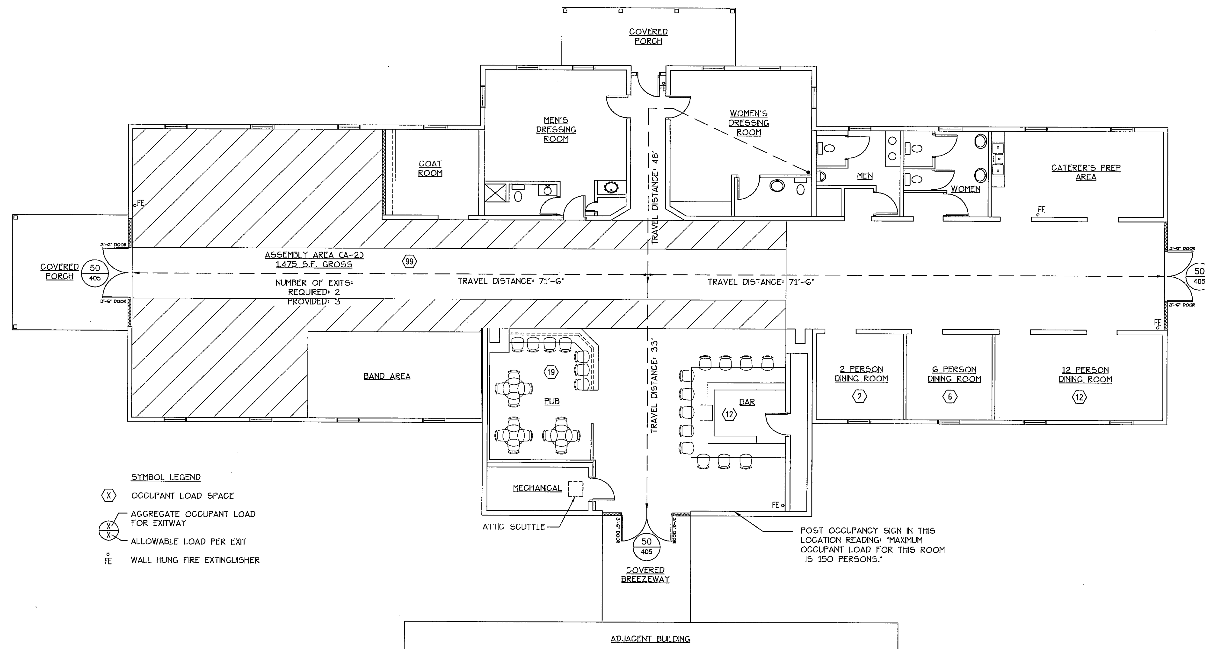
LIFE SAFETY PLAN SCALE: 1/8"=1'-0"
