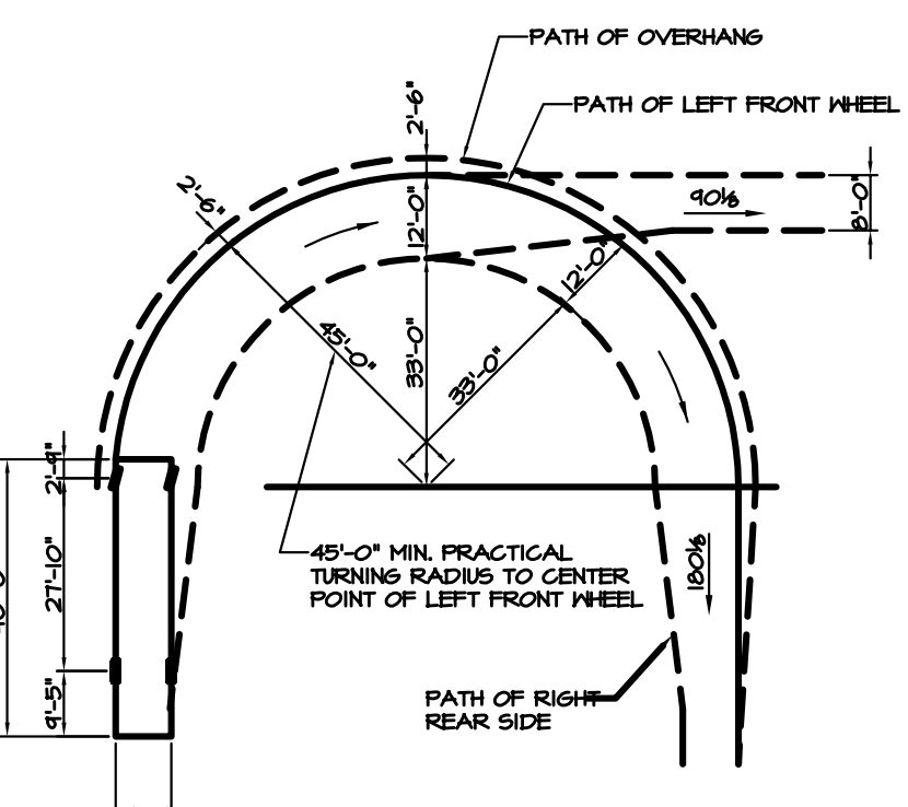
40'-0" STRAIGHT BODY RV MIN. PRACTICAL TURNING RADIUS OF 45'-0" 3 RADIUS DETAIL SDI N.T.S.
