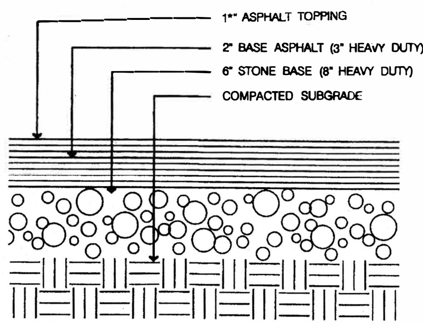
2 SPI TYPICAL PAVING SECTION NOT TO SCALE
