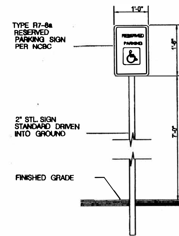
6 SPI HANDICAP SIGN NOT TO SCALE
