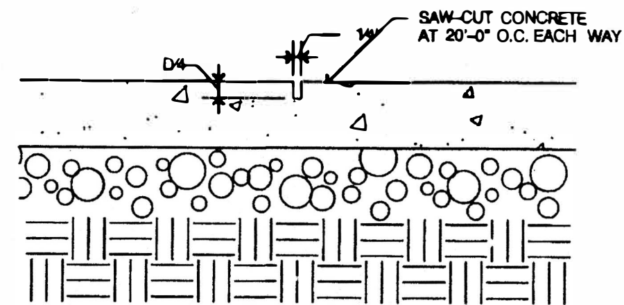
5 SPI CONTROL JOINT DETAIL NOT TO SCALE
