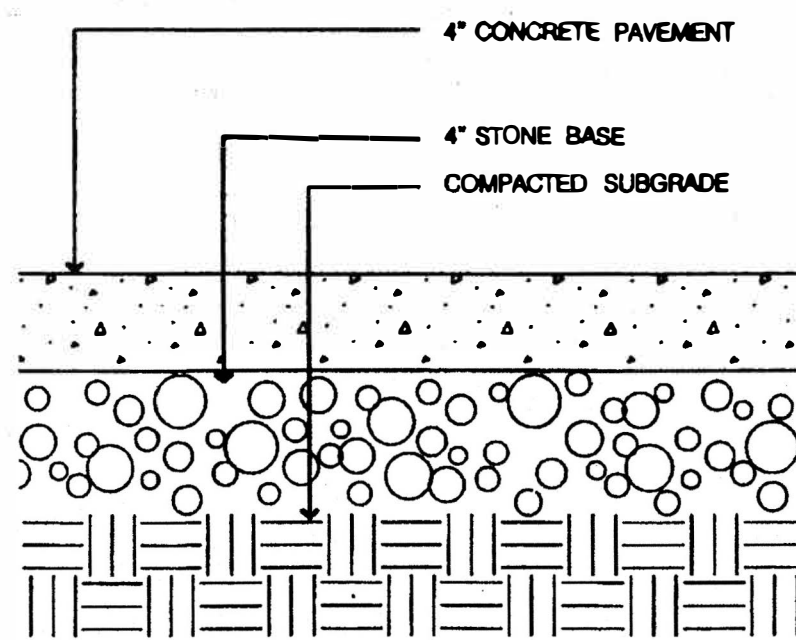
4 SPI TYPICAL SIDEWALK SECTION NOT TO SCALE
