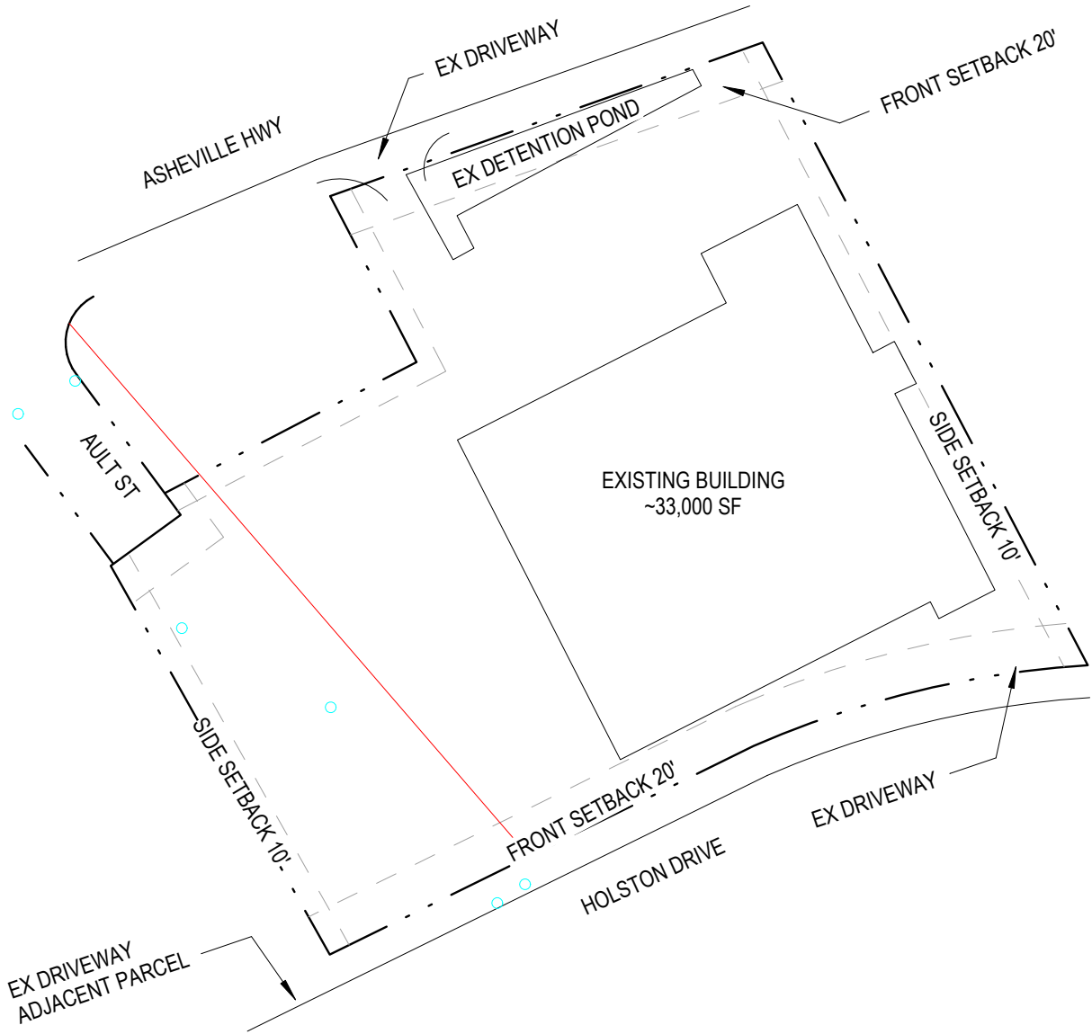
SITE PLAN 1" = 80'-0"
